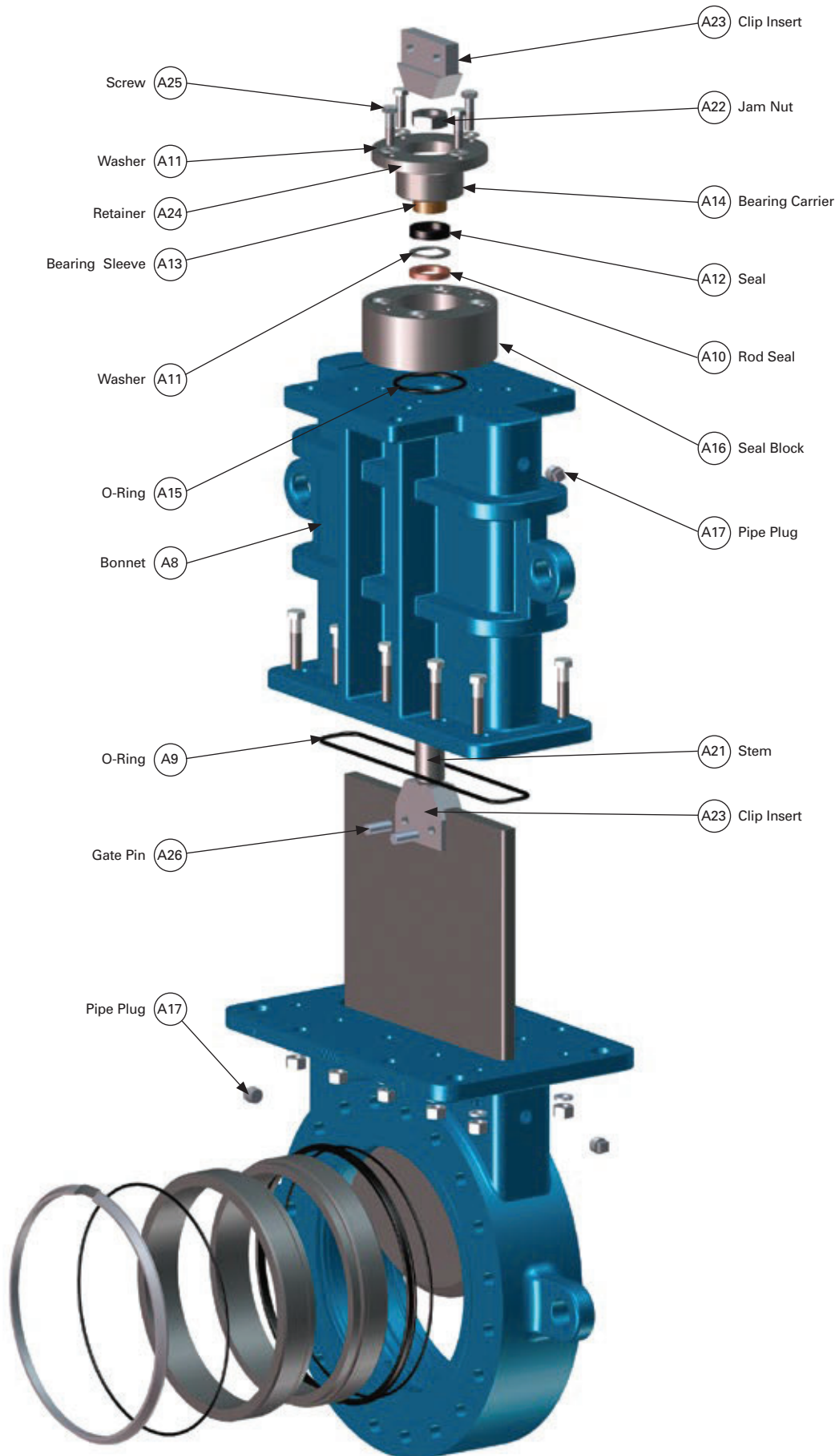
Class 150/300 Bonneted
