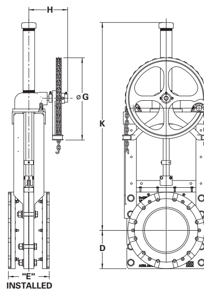
Standard Mounting
