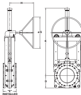
90 Degree Mounting
